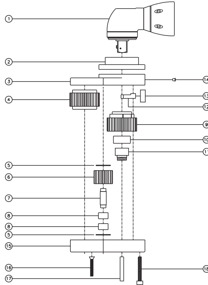
PARTS BLOWOUT
