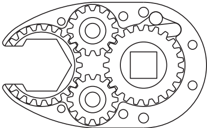
GEAR ASSEMBLY
