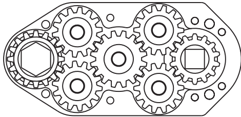
GEAR ASSEMBLY
