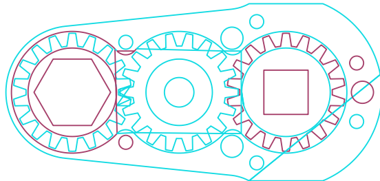
GEAR ASSEMBLY
